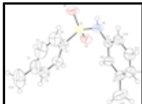
Fig. 1. Molecular structure of (I), showing the atom labelling scheme and displacement ellipsoids drawn at the 50% probability level.
